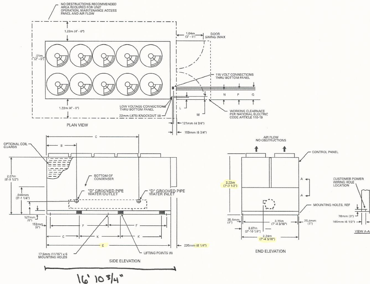
Figure D-1 — RTAA 70-125 Unit Dimensions
