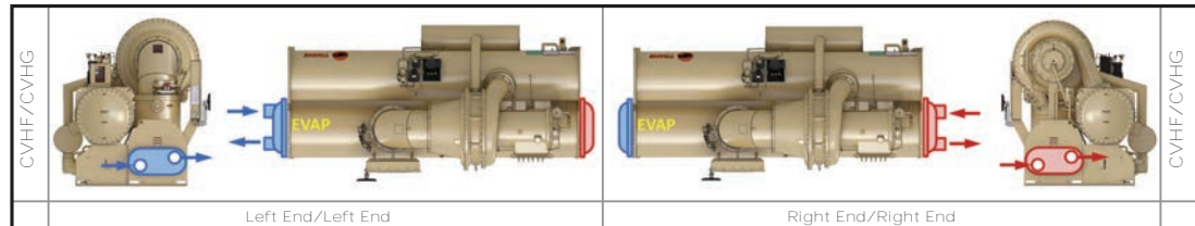
Figure 28. One-pass or three-pass non-marine evaporator waterbox configurations
