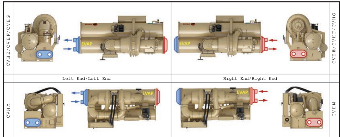
Figure 27. Two-pass non-marine evaporator waterbox configurations (250E only)
