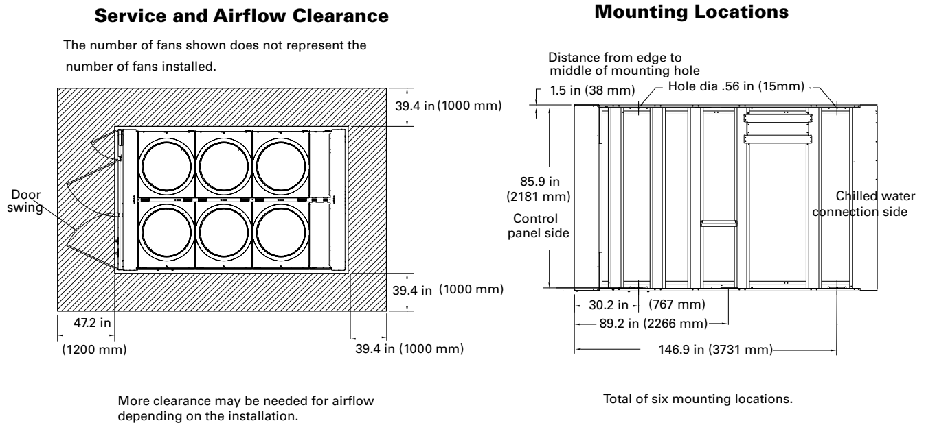
Figure 13. CGAM 100, 110 and 120 ton — service clearances and mounting locations
