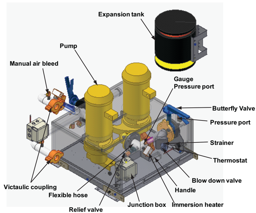
Figure 53. Pump package components, slant 20-35T, view 1
