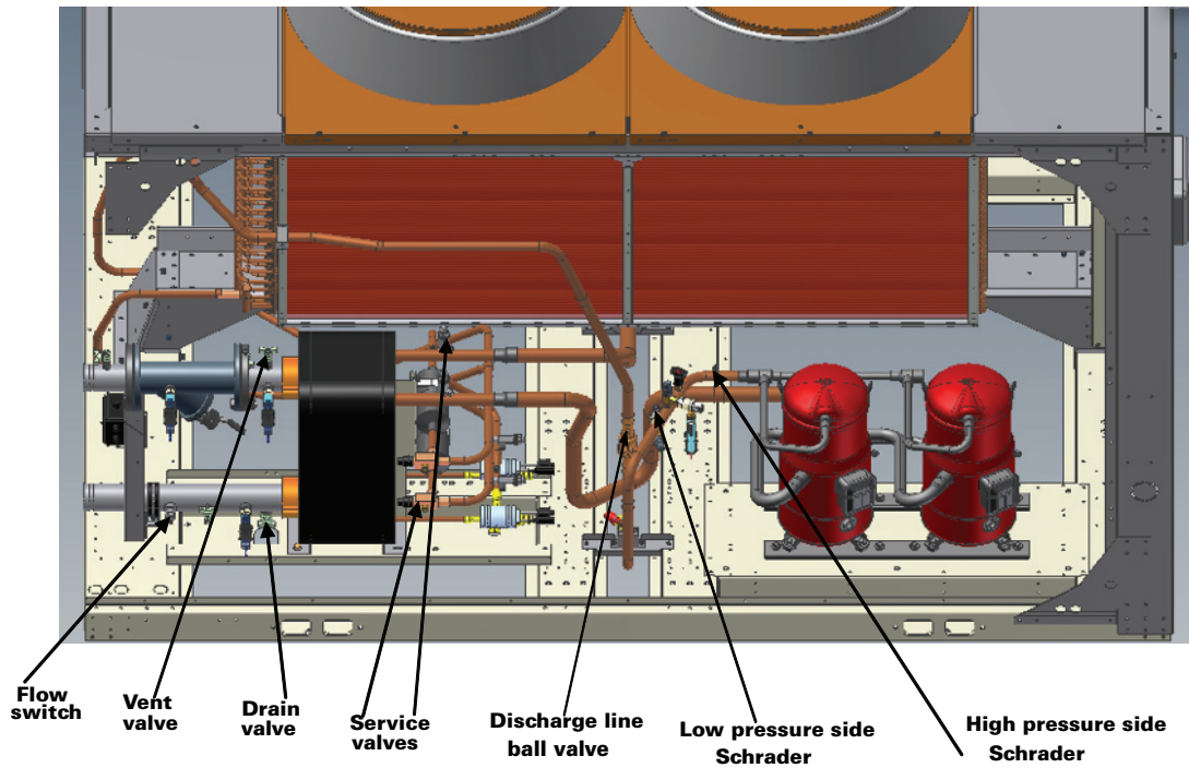
Figure 51. W 80-130 ton component location - compressor view
