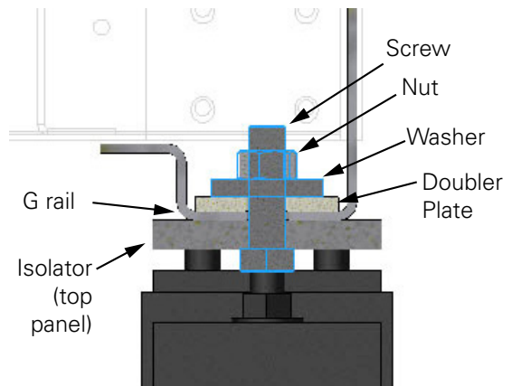
Figure 23. Seismic isolator installation detail
