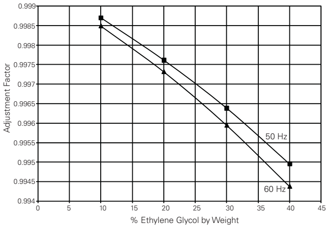
Figure 31. Propylene - compressor power adjustment
