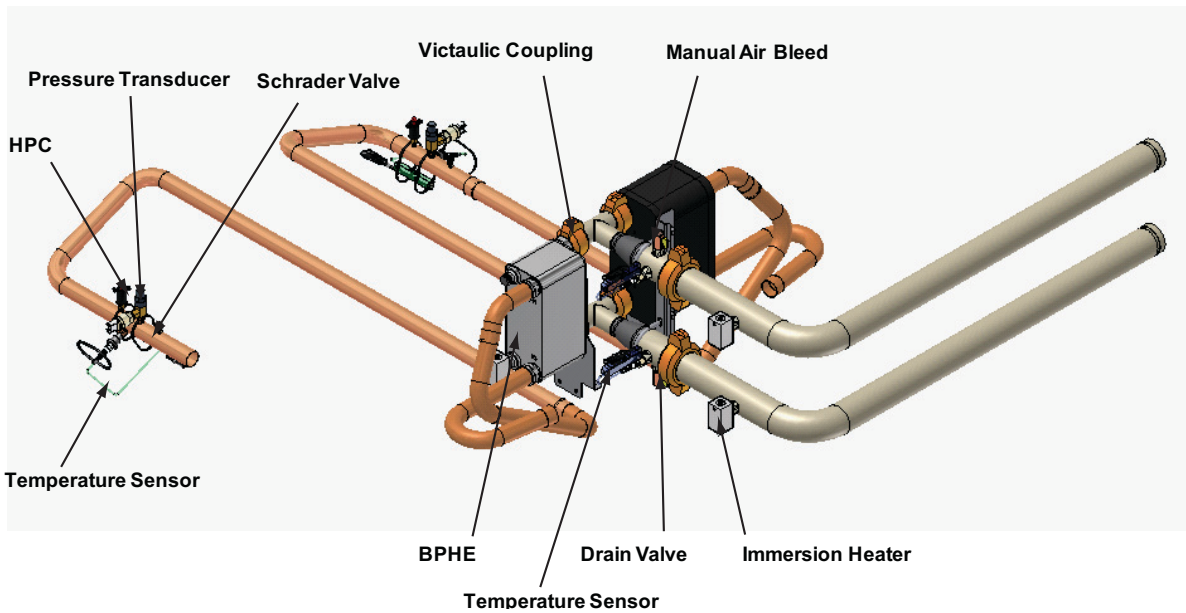
Figure 63. Partial heat recovery components – W 80-130 ton
