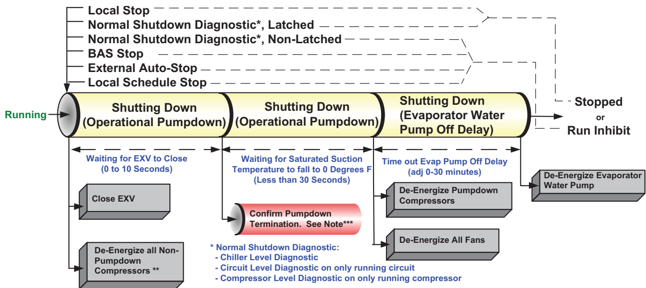
Figure 81. Normal shutdown to stopped or run inhibit
