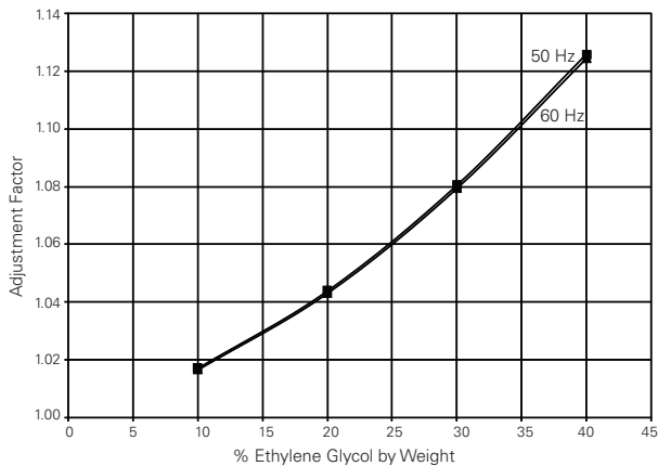
Figure 32. Ethylene - GPM adjustment
