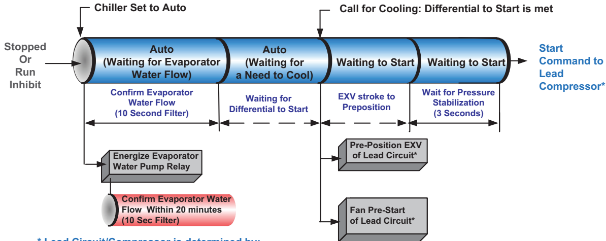
Figure 80. Stopped to starting
