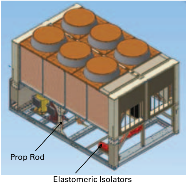
Figure 7. Ship with location — isolator and prop rod W 80-130 ton - s
