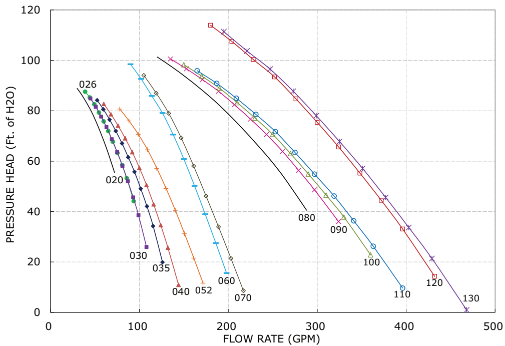
Figure 46. CGAM pump package available head pressure - water only
