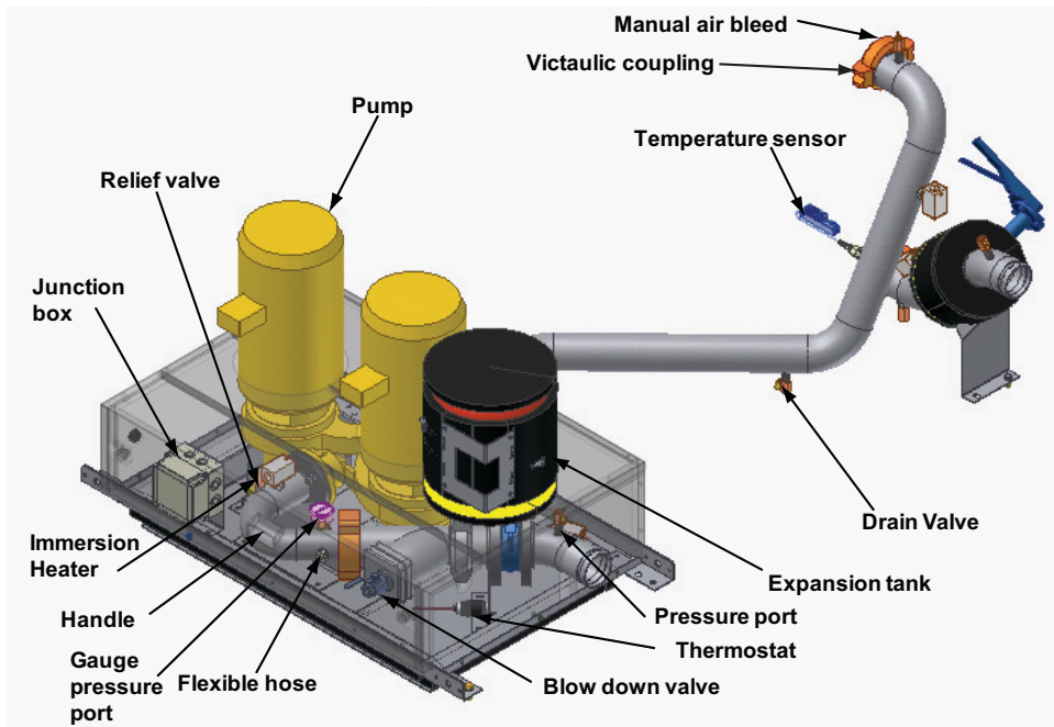
Figure 55. Pump package components, V40-70T, view 1
