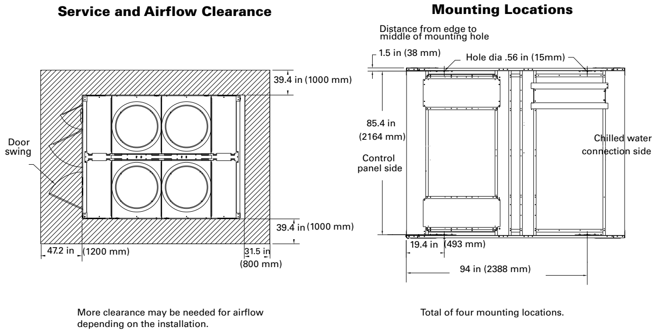
Figure 11. CGAM 60 and 70 ton - service clearances and mounting locations
