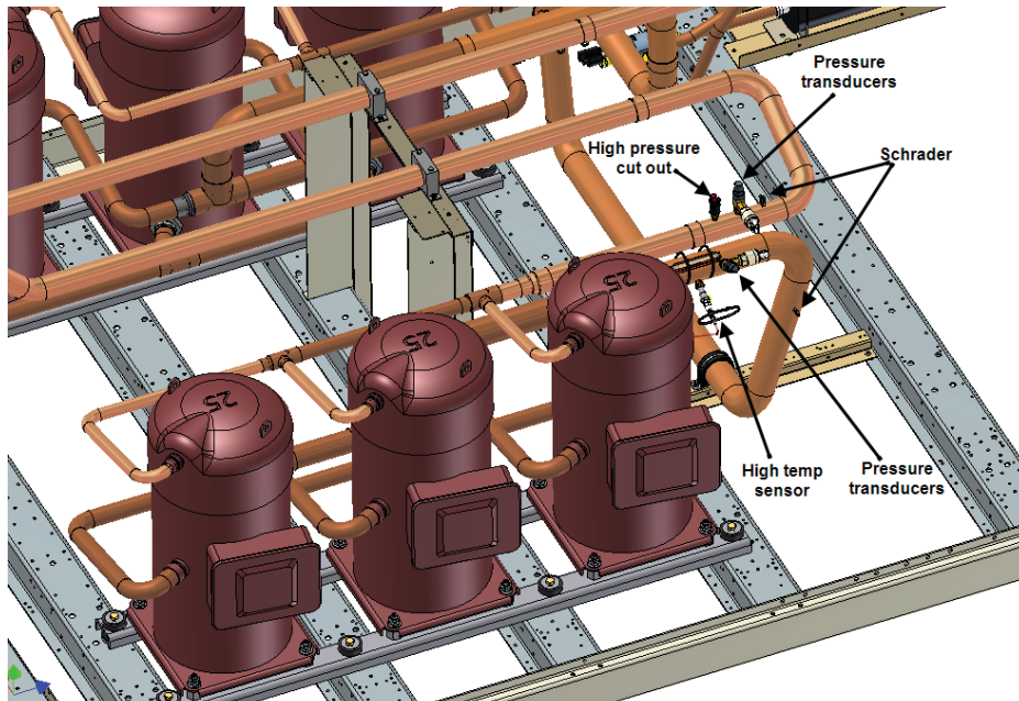
Figure 51. W 80-130 ton component location - compressor view
