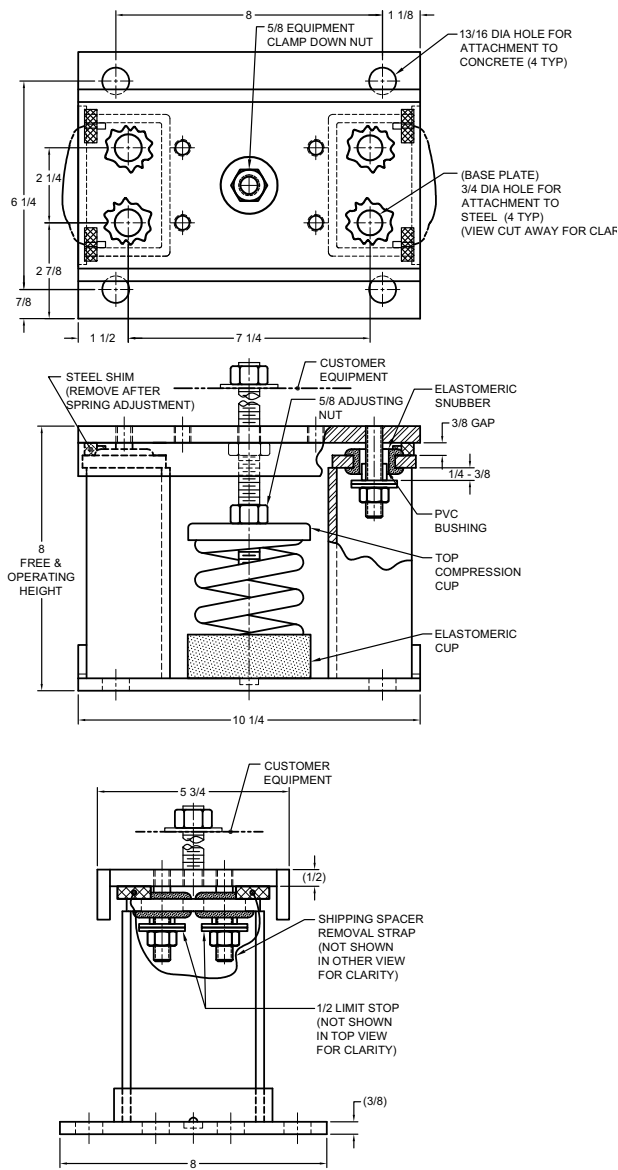
Figure 19. MSSH seismically rated isolator
