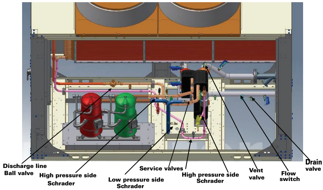
Figure 48. Slant 20-35 ton component location
