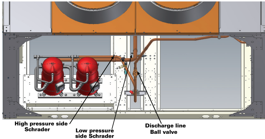
Figure 49. V 40-70 ton component location - circuit 1
