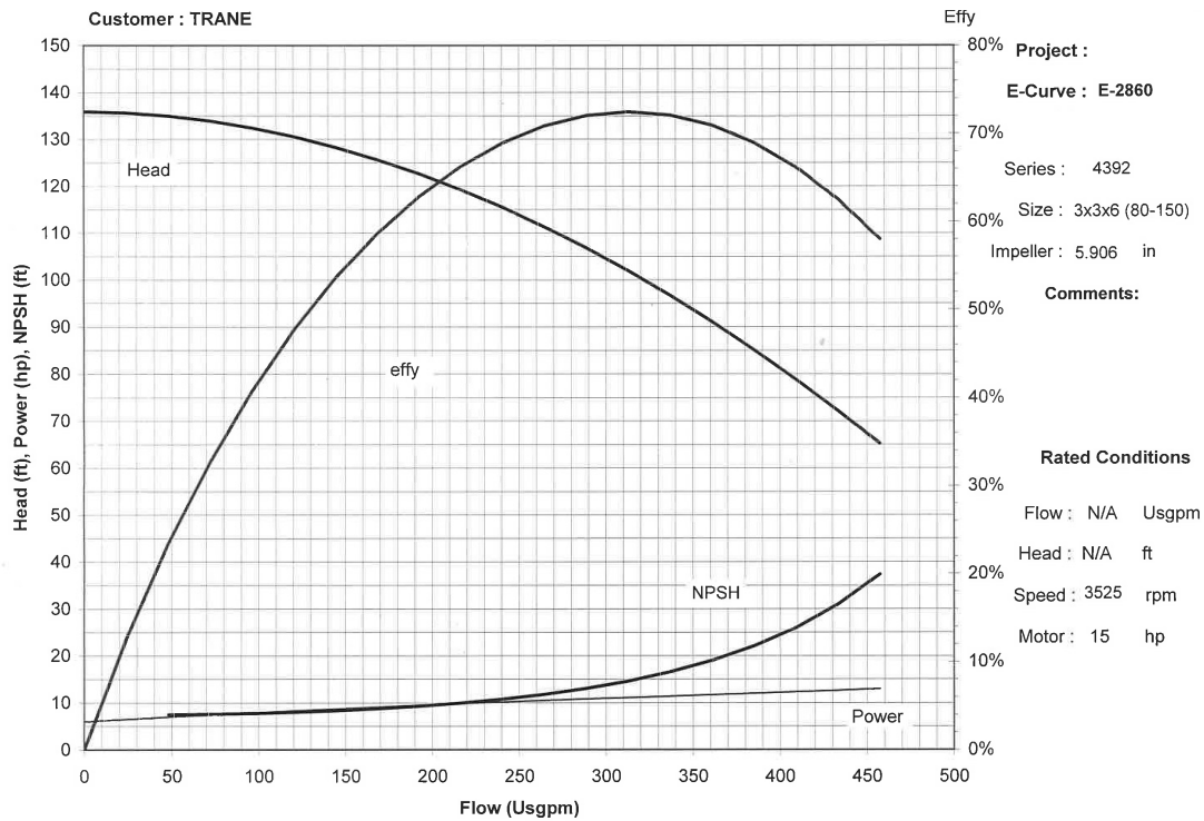
Figure 44. Pump curve - 120-130T - water only
