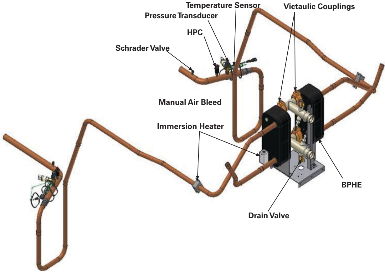
Figure 62. Partial heat recovery components, V40-70T
