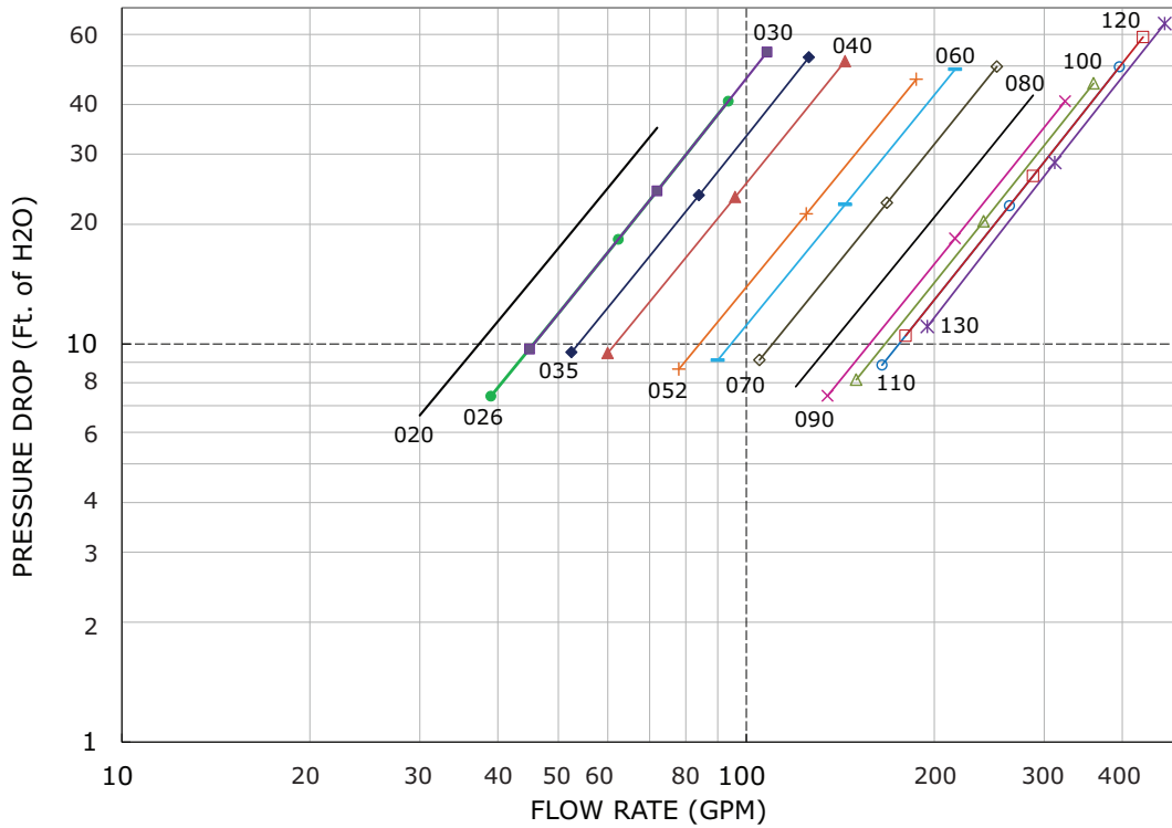
Figure 45. Unit component pressure drop - water only
