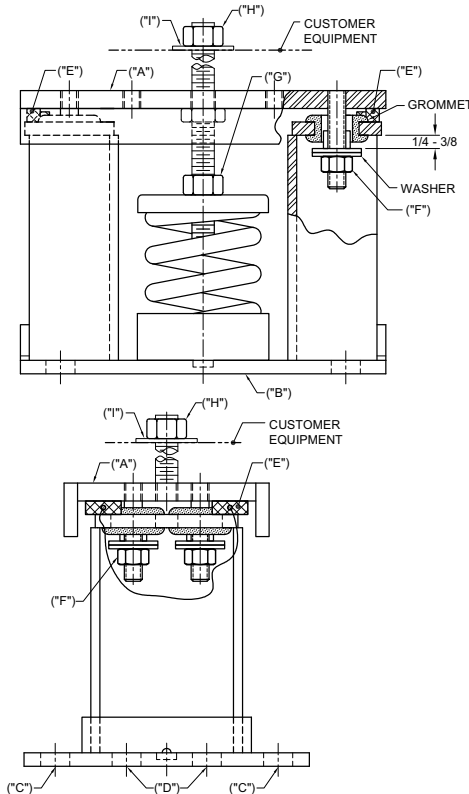
Figure 22. M2SS seismic isolator installation reference
