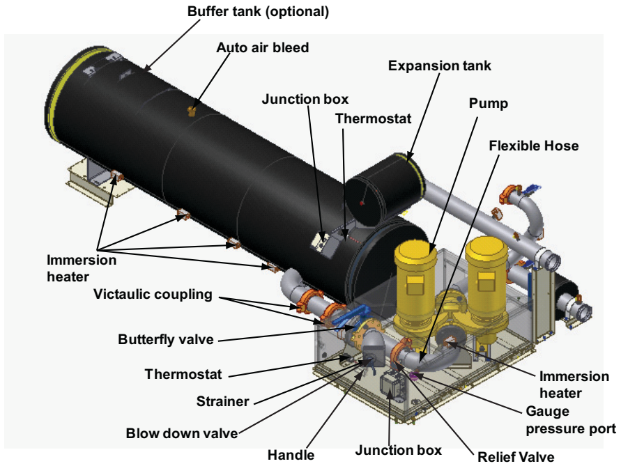
Figure 58. Pump package components – W 80-130 ton – view 1
