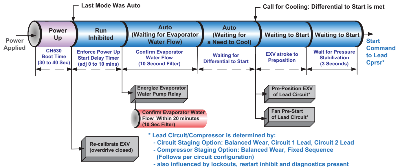
Figure 79. Power up to starting
