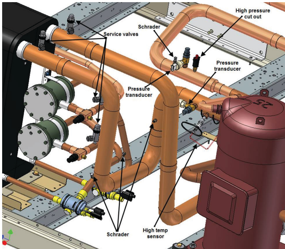
Figure 52. W 80-130 ton component location - evaporator side
