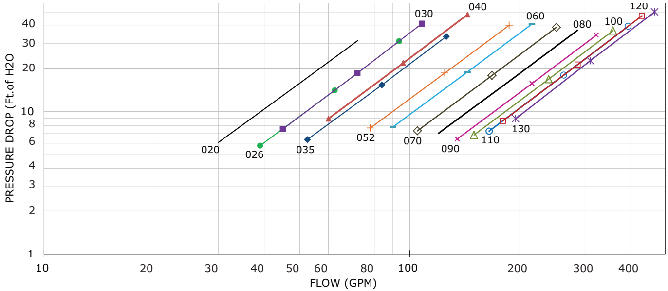
Figure 28. Total unit pressure drop curves (60 Hz)
