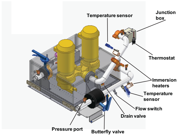
Figure 54. Pump package components, slant 20-35T, view 2
