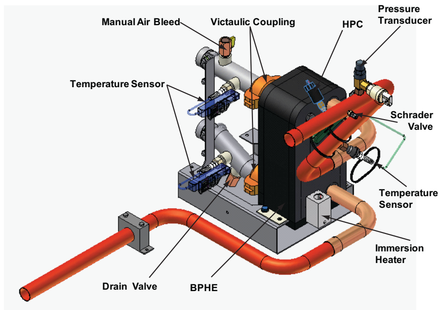
Figure 61. Partial heat recovery components, slant 20-35T
