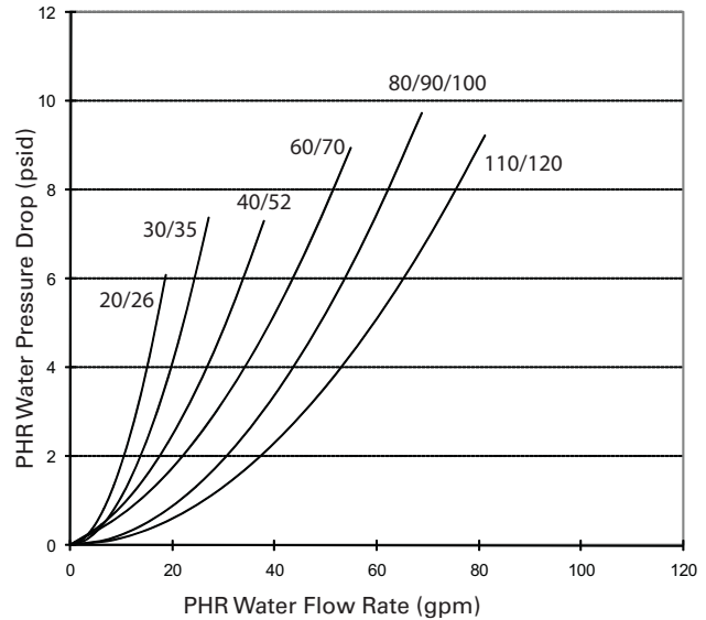
Figure 38. Partial heat recovery pressure drop curve — 50 Hz
