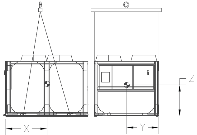
Figure 16. CGAM V 40-70 ton rigging
