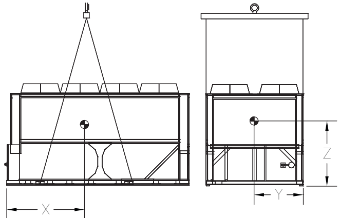
Figure 17. CGAM W 80-130 ton rigging
