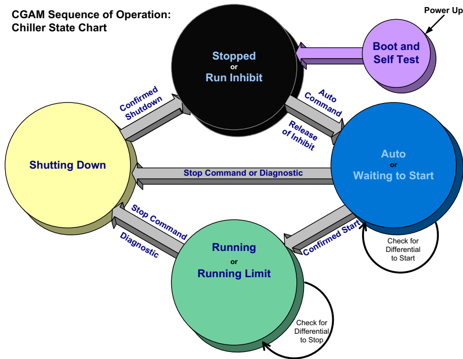
Figure 77. Chiller state chart
