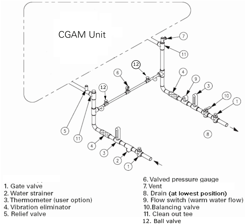
Figure 36. Partial heat recovery piping recommendations
