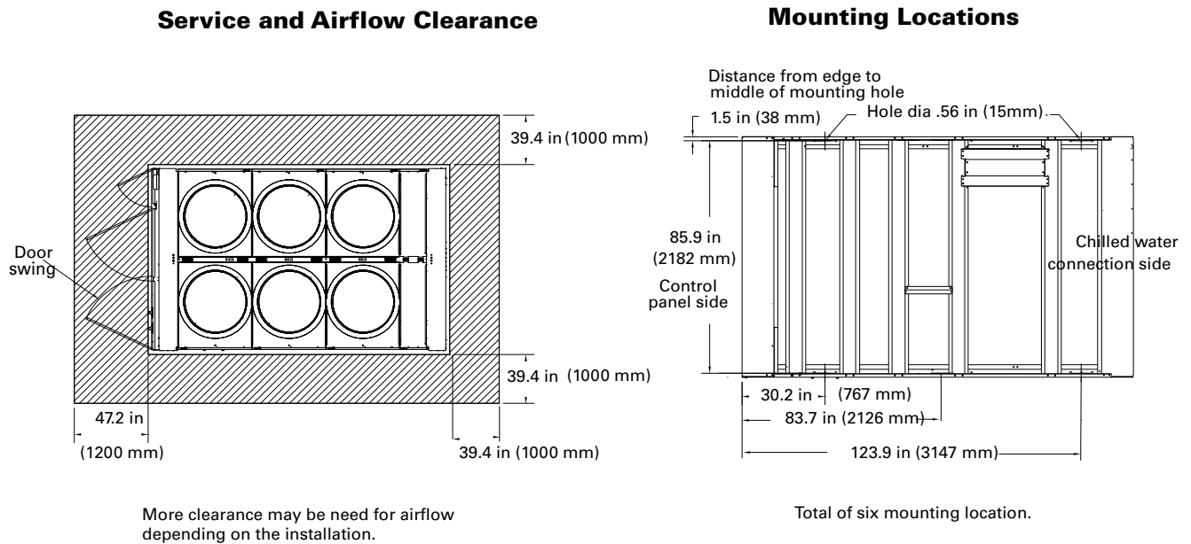
Figure 12. CGAM 80 and 90 ton - service clearances and mounting locations
