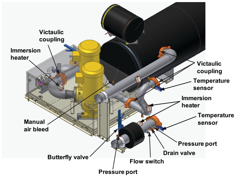
Figure 59. Pump package components – W 80-130 ton – view 2
