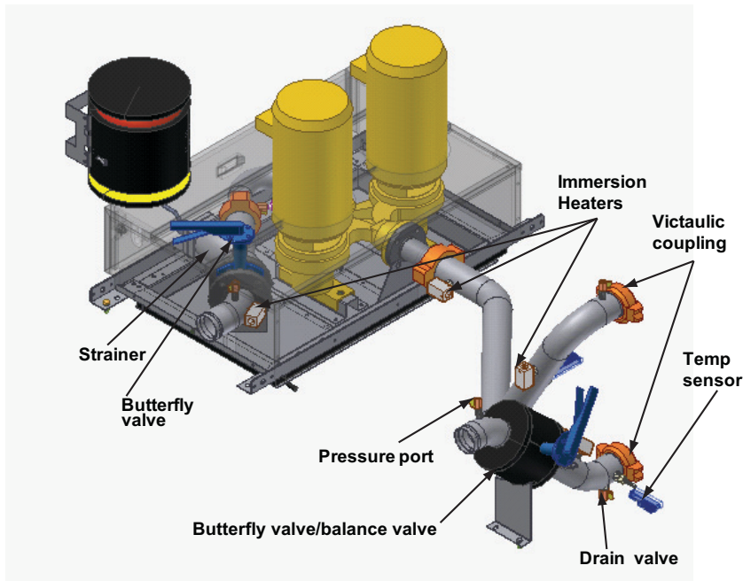
Figure 56. Pump package components, V40-70T, view 2
