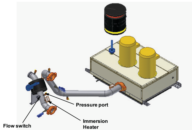
Figure 57. Pump package components – V 40-70 ton – view 3
