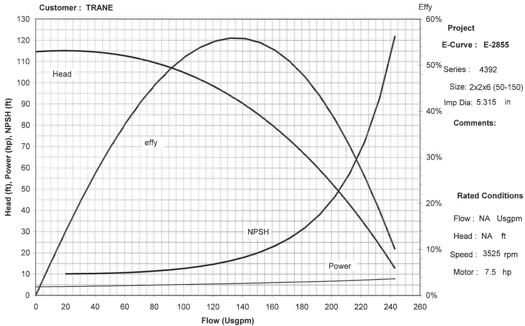
Figure 42. Pump curve - 60-70T - water only
