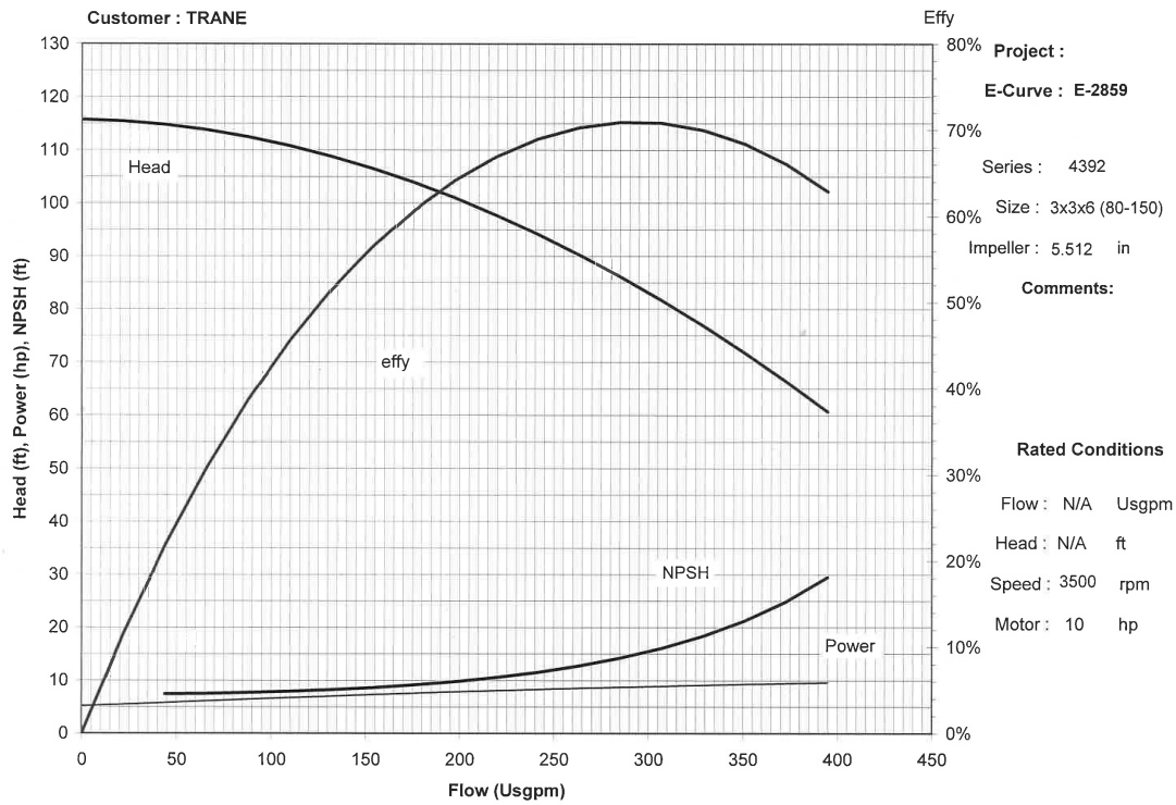
Figure 44. Pump curve - 120-130T - water only
