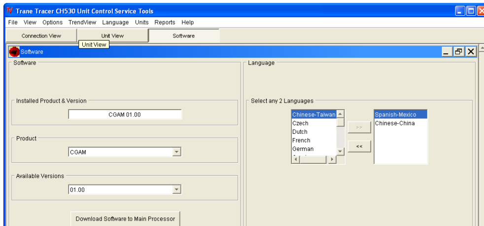
Figure 75. Software view
