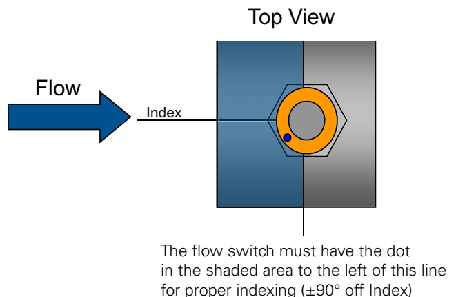
Figure 26. Proper flow switch indexing
