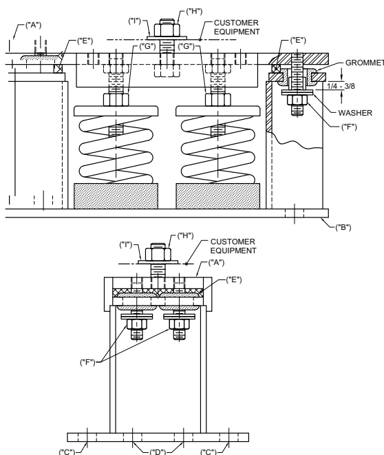
Figure 22. M2SS seismic isolator installation reference
