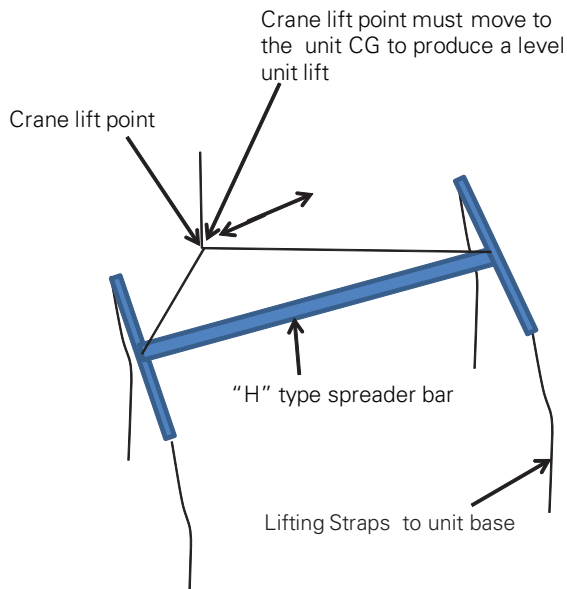
Figure 14. H-type spreader bar adjustment for level unit lift
