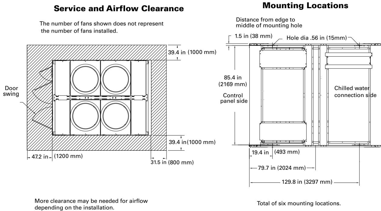
Figure 11. CGAM 60 and 70 ton - service clearances and mounting locations
