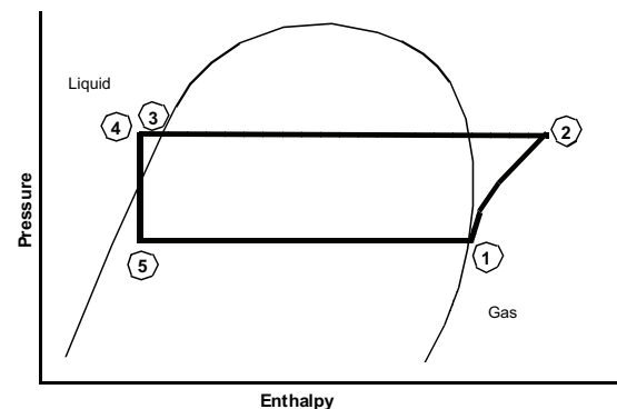
Figure 64. Pressure/enthalpy curve
