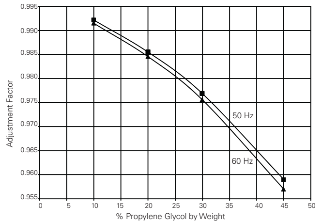
Figure 35. Propylene - capacity adjustment
