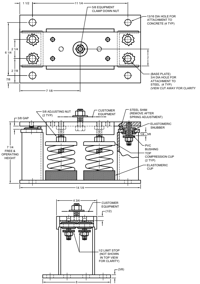
Figure 20. M2SS seismically rated isolator
