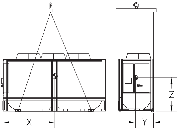
Figure 15. CGAM slant 20-35 ton rigging
