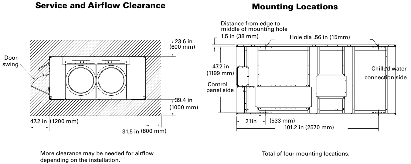
Figure 9. CGAM 30 and 35 ton — service clearances and mounting locations
