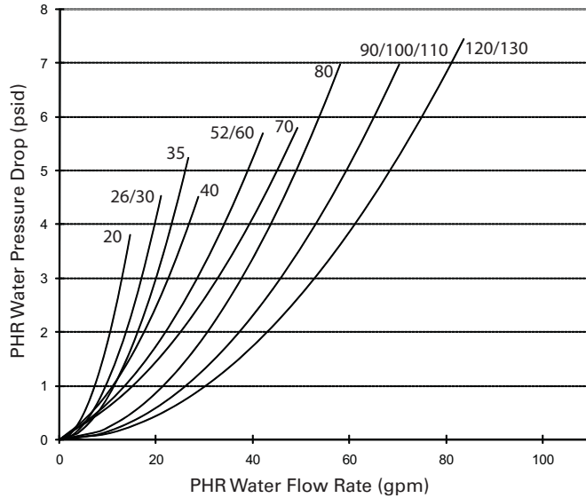
Figure 37. Partial heat recovery pressure drop curve — 60 Hz
