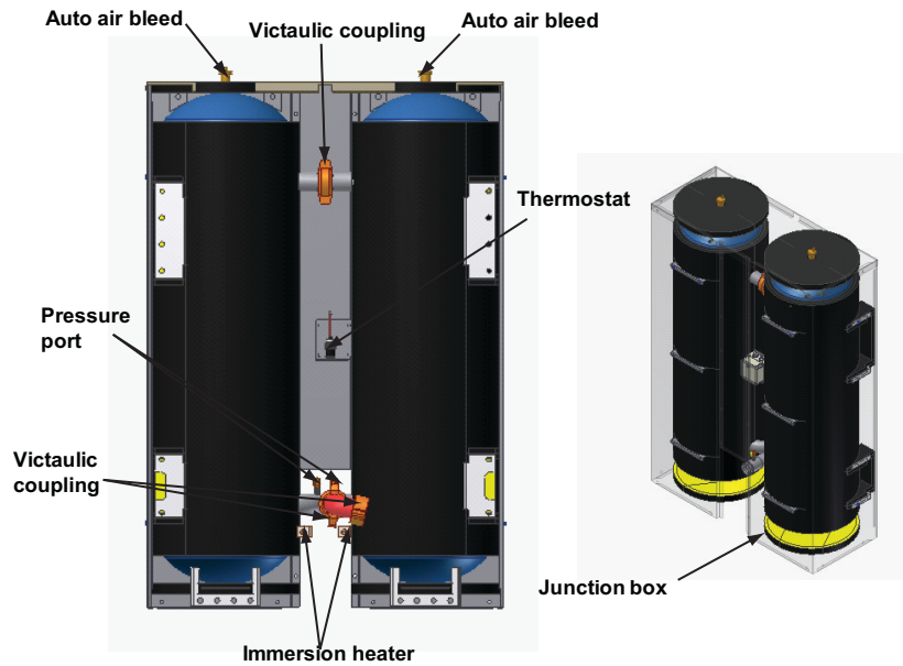
Figure 60. Buffer tank components — slant 20-35 ton & V 40-70 ton
