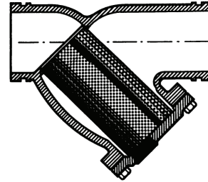
Figure 83. Y type strainer — units with optional pump package
