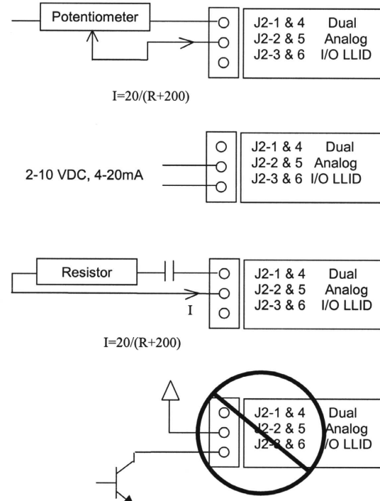
Figure 47. Wiring examples for ECLS and EDLS
