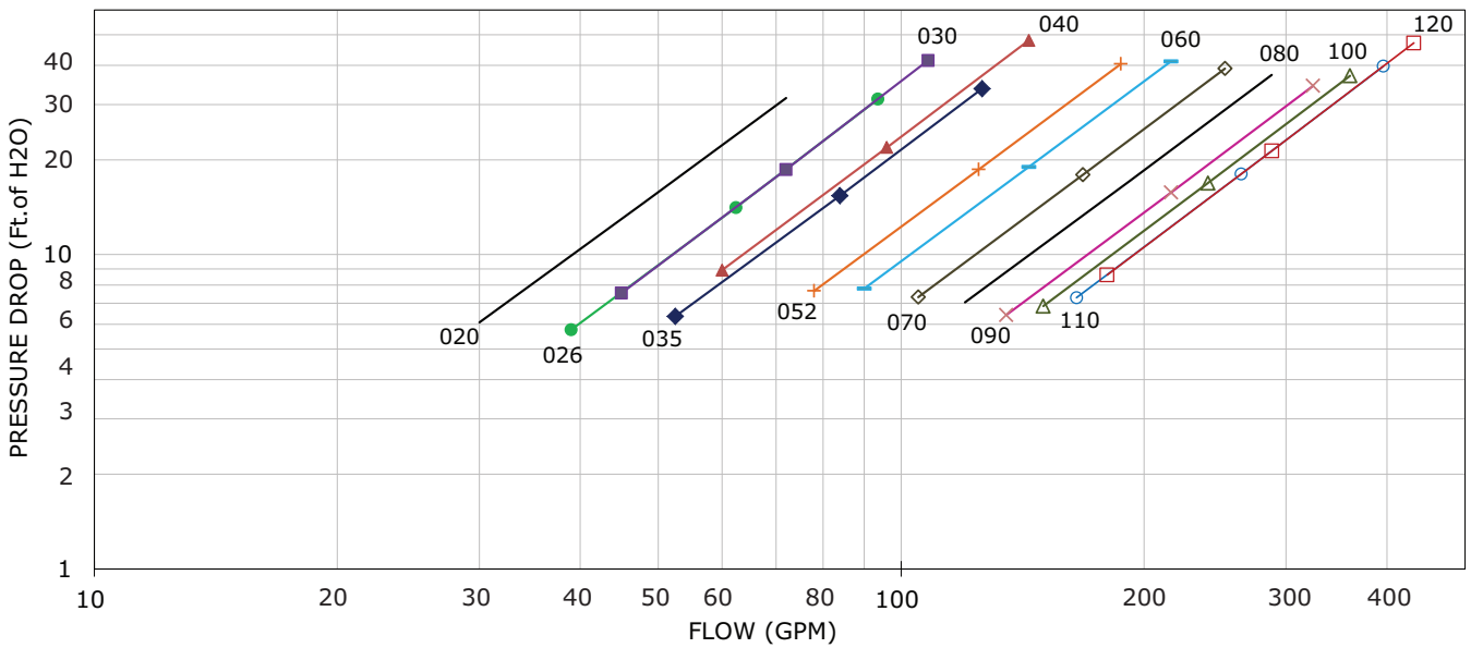
Figure 29. Total unit pressure drop curves (50 Hz)
