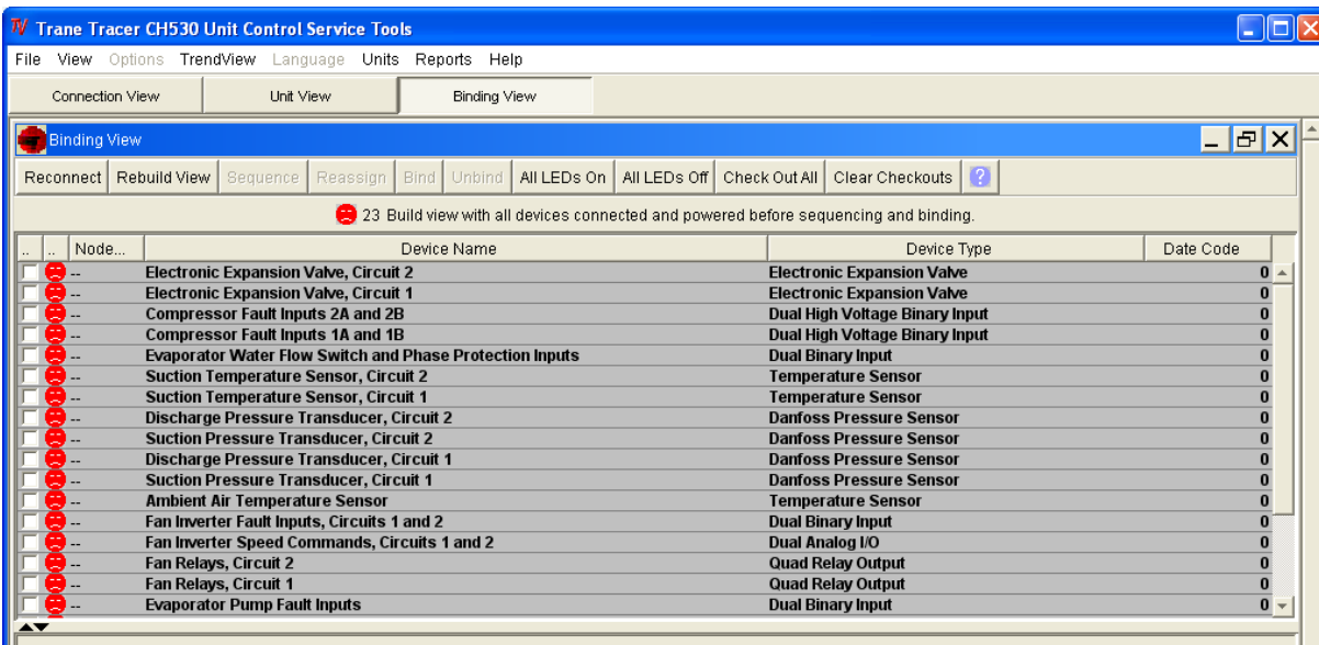
Figure 76. Binding view
