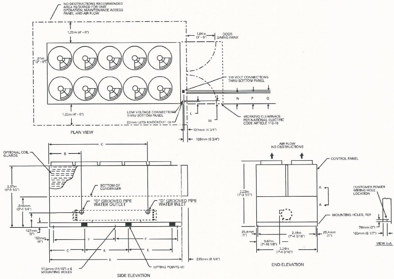
Figure D-1 — R 'AA 70-125 Unit Dimensions
