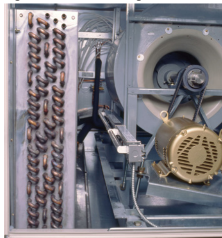
Figure 19: Ultraviolet Light
