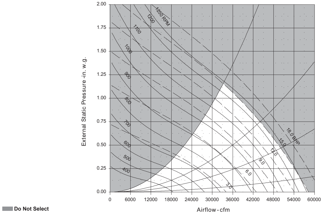
Figure 76: RPS/RFS/RDT 080D to 140D (3) 36 in. Propeller Exhaust Fan
