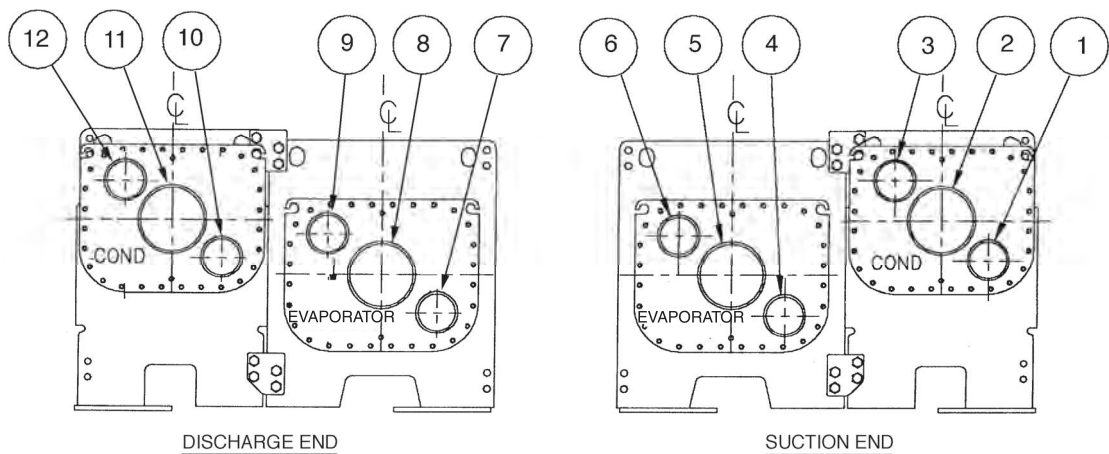
FRAME 3
