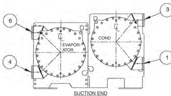
FRAMES 4, AND 5
