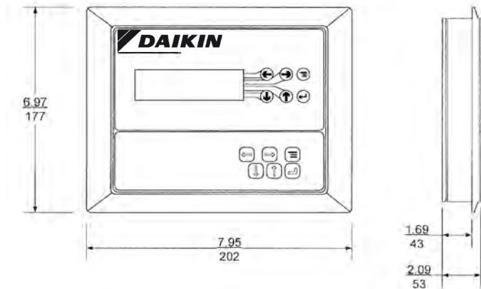
Figure 5, Remote Interface Panel Dimensions
