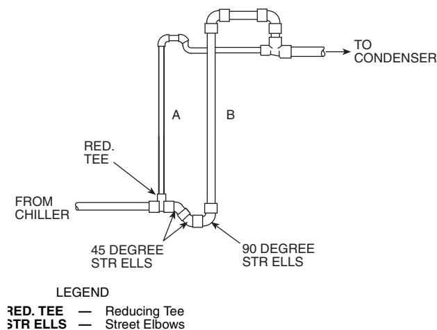
Fig. 17 — Double Discharge Riser Construction Detail
