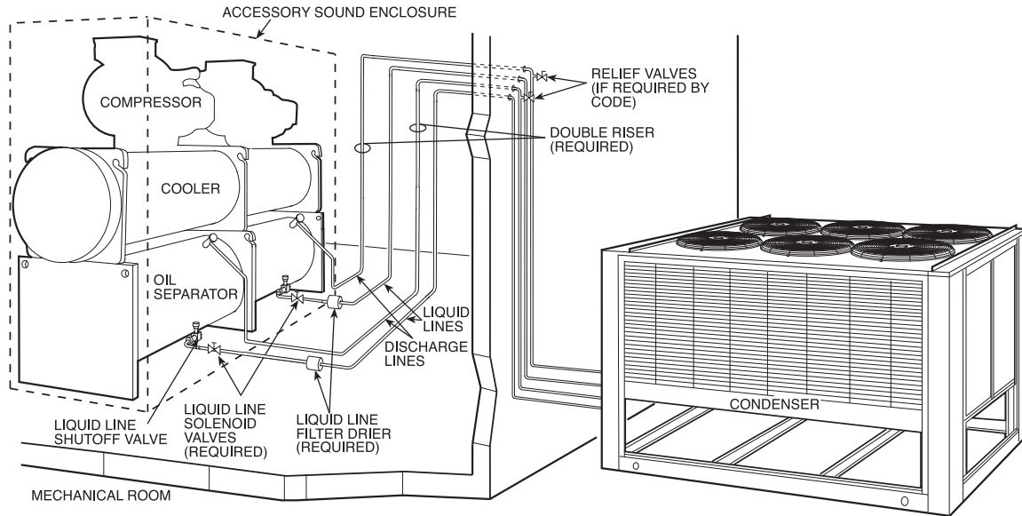
Fig. 14A — Typical 30HXA Refrigerant Piping to Remote Condenser (076-096 Sizes Shown)
