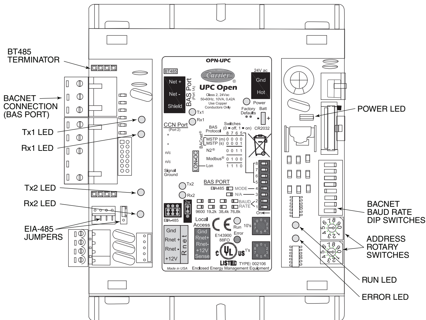
Fig. 22 — UPC Open Controller
