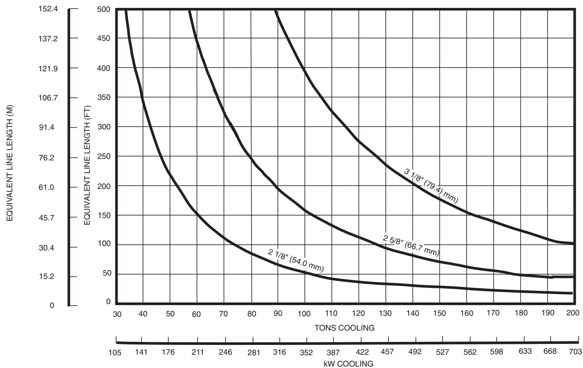
Fig. 15 — R-134a Liquid Line Sizing, 30HXA Units
