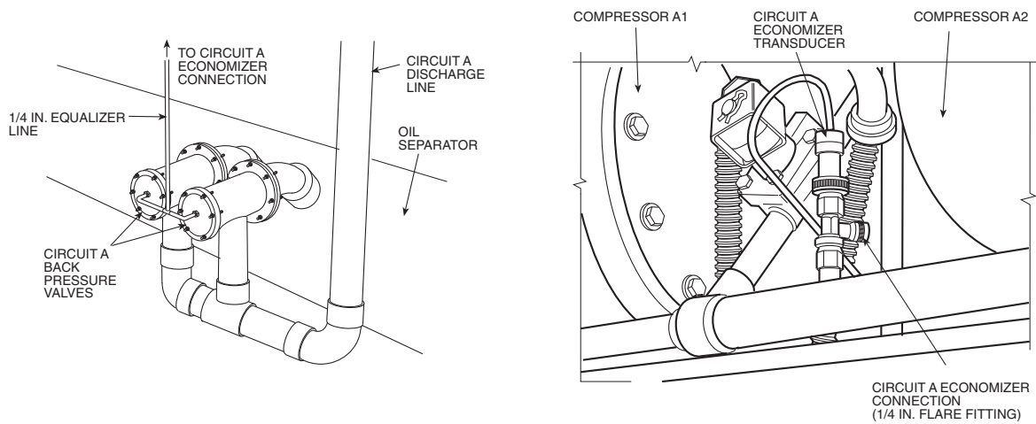
Fig. 20 — 30HXA206-271 Back Pressure Valve Equalizer Line Connection (Circuit A)
