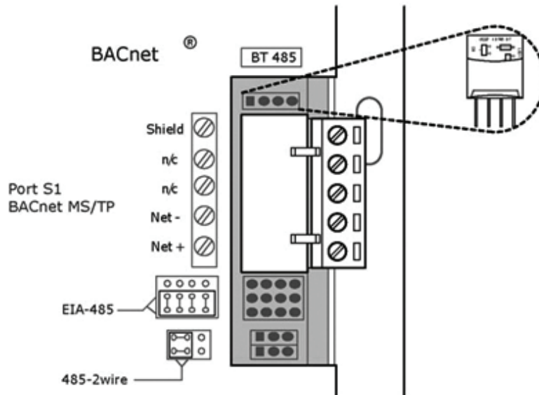
Fig. 24 — BT485 Terminator Installation
