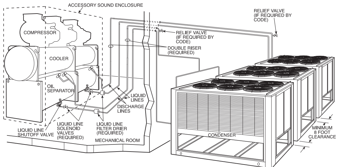
Fig. 14B — Typical 30HXA Refrigerant Piping to Remote Condenser(s) (206-271 Sizes Shown)
