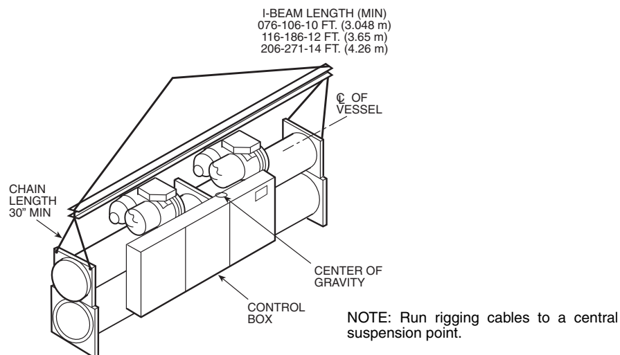
Fig. 12 — Unit Rigging (Size 076-186 Shown, Larger Sizes Similar)
