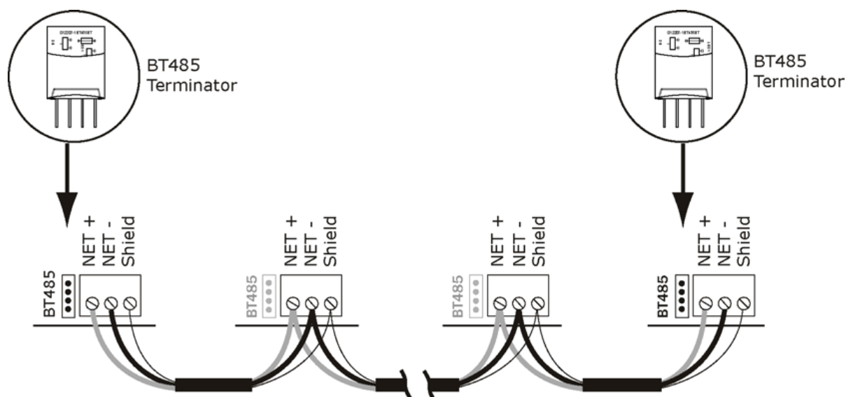
Fig. 23 — Network Wiring
