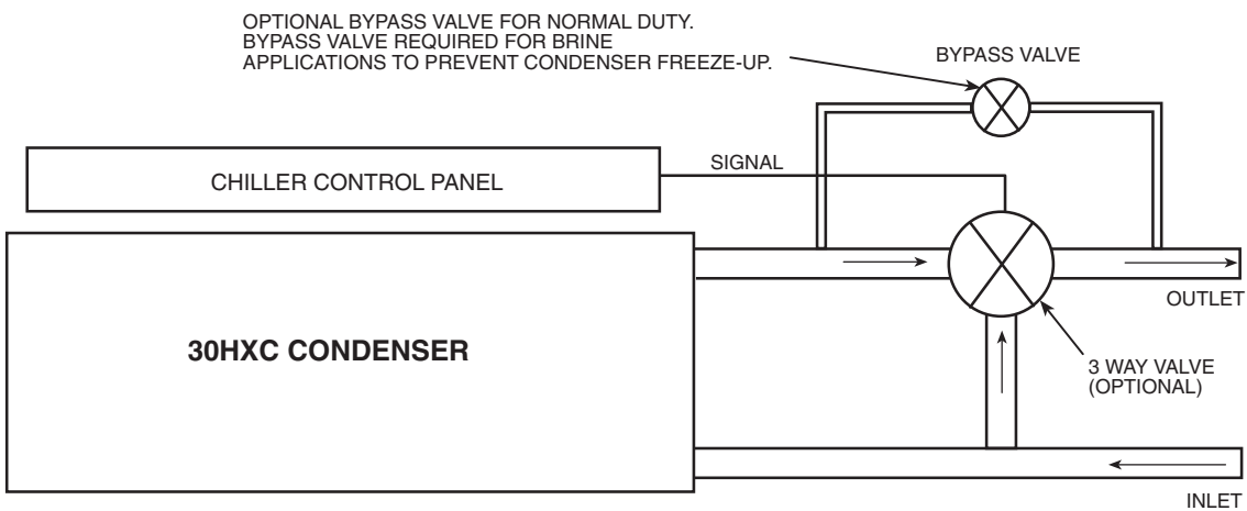
Fig. 21 — Condenser Temperature Regulating Valve Installation
