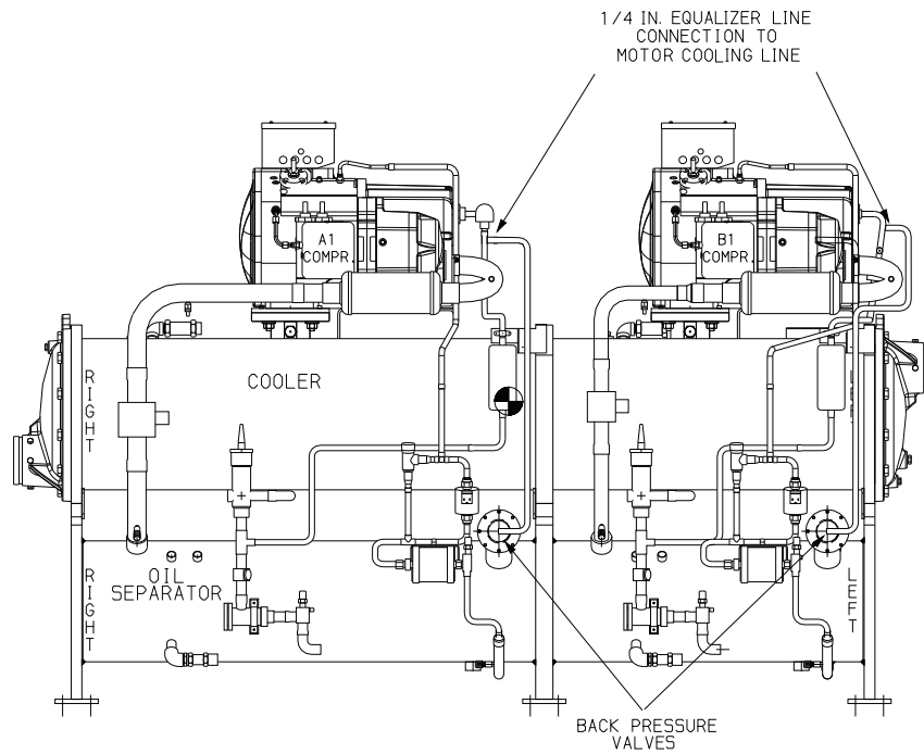
Fig. 19 — 30HXA Units Back Pressure Valve Equalizer Line Connection (076-186 Sizes Shown)
